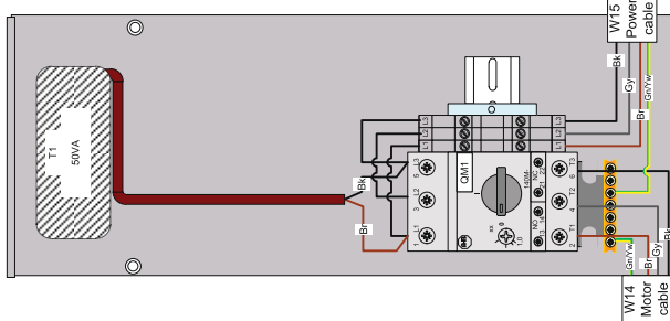
Filterbox Basic Wiring diagram 3P 200-240V IEC 2162482 3P 380-420V IEC 2162483
