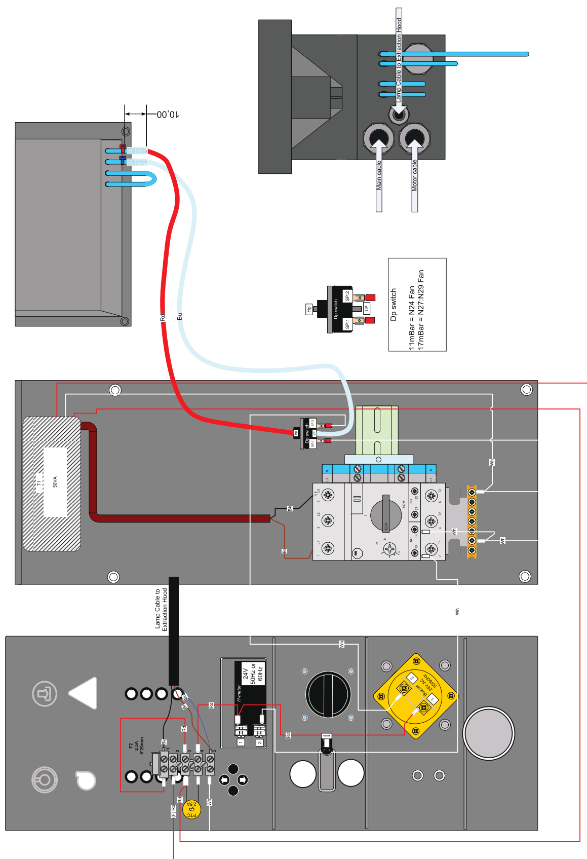
FilterBox Basic III, Layout Control Cable Basic IEC / UL-CSA
